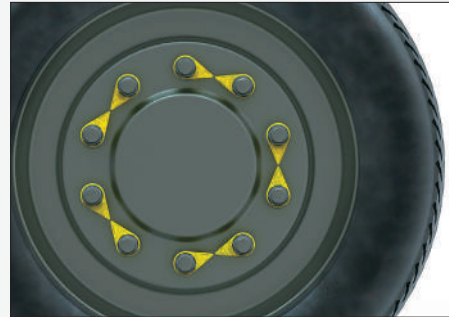
The Checkpoint Loose Wheel Nut Indicators in use.
