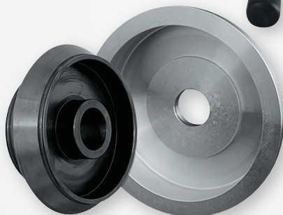
483-40091 Light Truck Cone Kit 40mm
